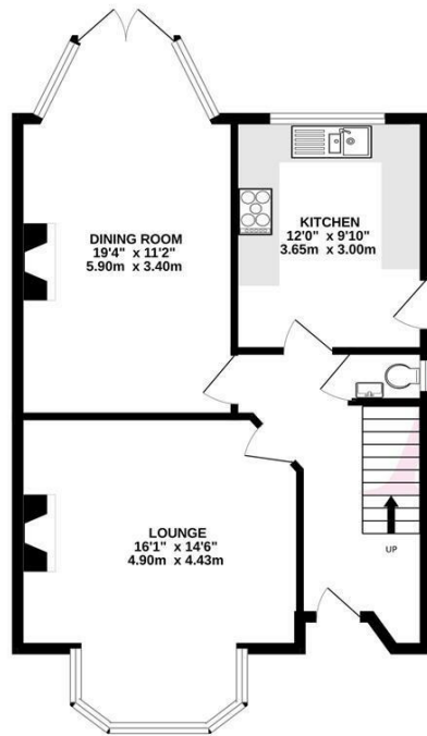
GROUND FLOOR 742 sq.ft. (69.0 sq.m.) approx.
