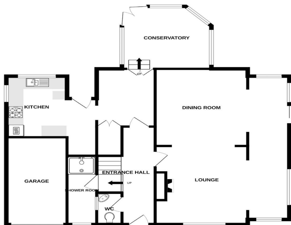
GROUND FLOOR 97.0 sq.m. (1044 sq.ft.) approx.
