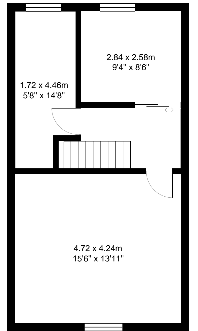
First Floor Area: 41.8 m 2 ... 450 ft 2
