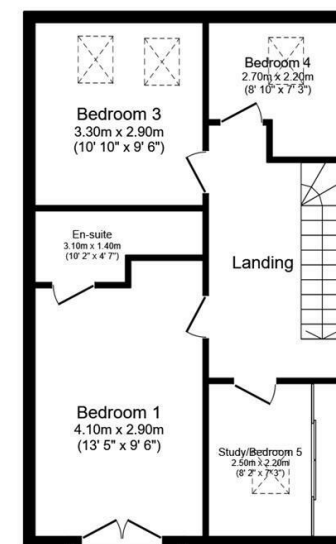
Second Floor Floor area 54.1 sq.m. (583 sq.ft.)
