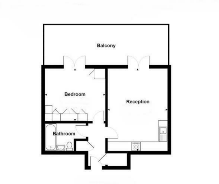
Total Area: 47.2 m² ... 508 ft² (excluding balcony) All measurements are approximate and for display purposes only
