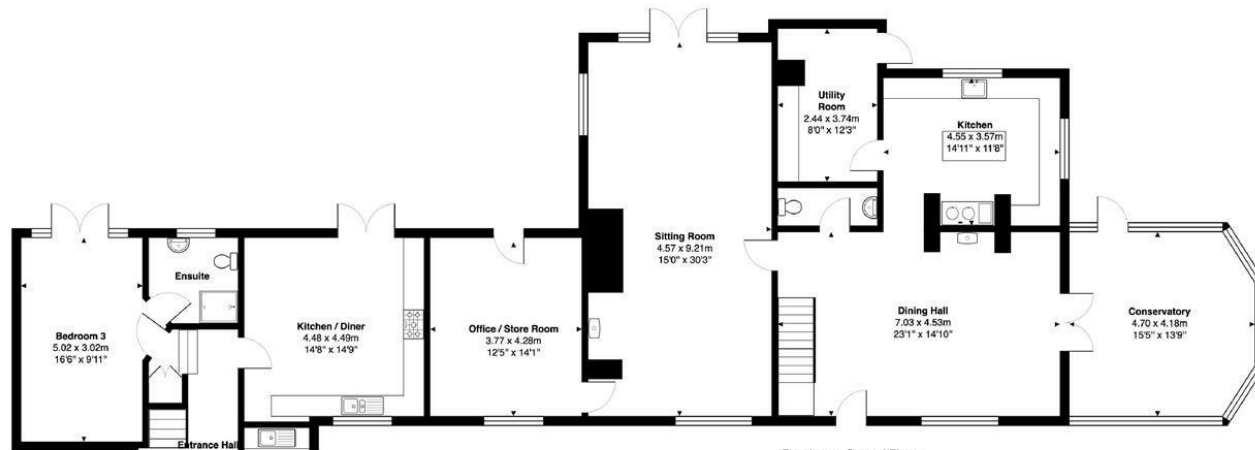
Farmhouse Ground Floor Area: 228.5 m² ... 2459 ft²
