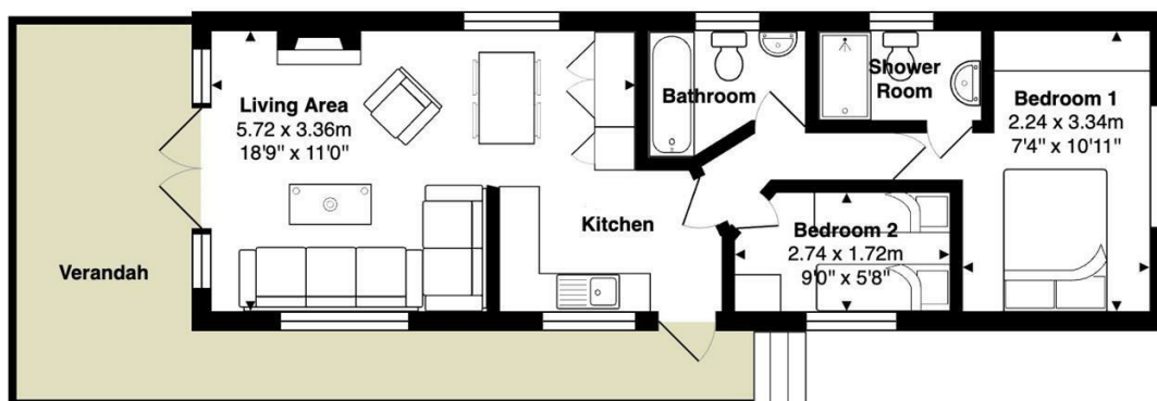
Ground Floor
