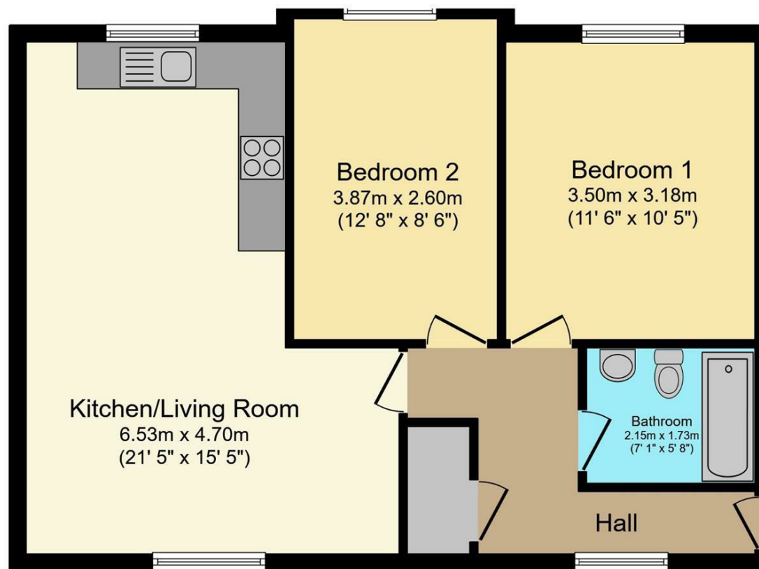
Floor Plan
