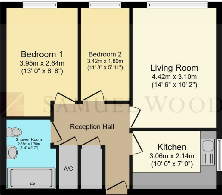
Floor Plan
