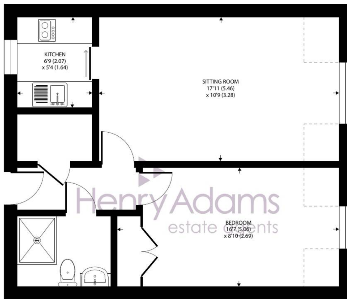
SECOND FLOOR
