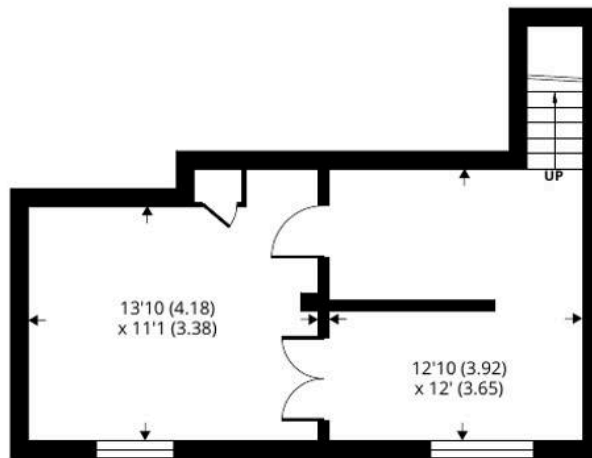
BASEMENT FLOOR
