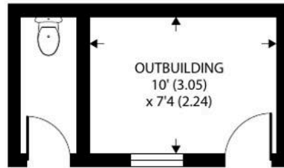
OUTBUILDING
