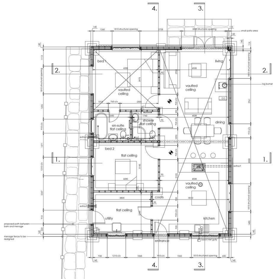
ground floor plan proposed scale 1:50
