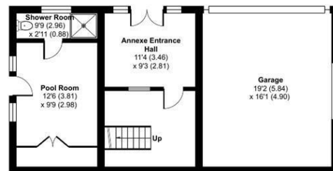
ANNEXE GROUND FLOOR / OUTBUILDING / GARAGE
