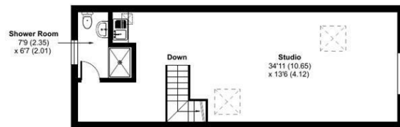
ANNEXE FIRST FLOOR
