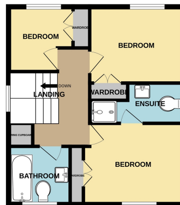
1ST FLOOR 448 sq.ft. (41.6 sq.m.) approx.
