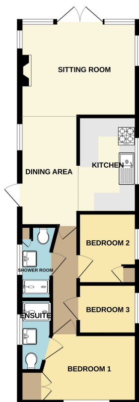
GROUND FLOOR 521 sq.ft. (48.4 sq.m.) approx.
