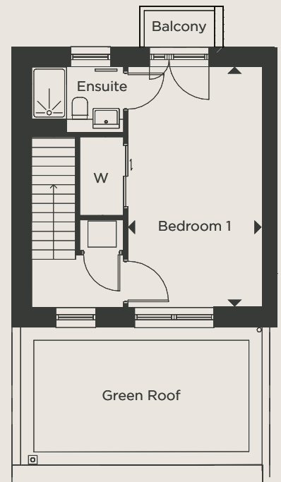
2ND FLOOR
