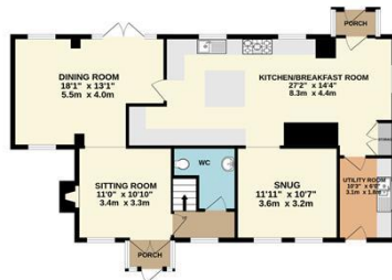
TOTAL FLOOR AREA : 2830 sq.ft. (263.0 sq.m.) approx.
