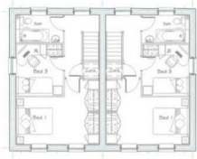
FIRST FLOOR LAYOUT
