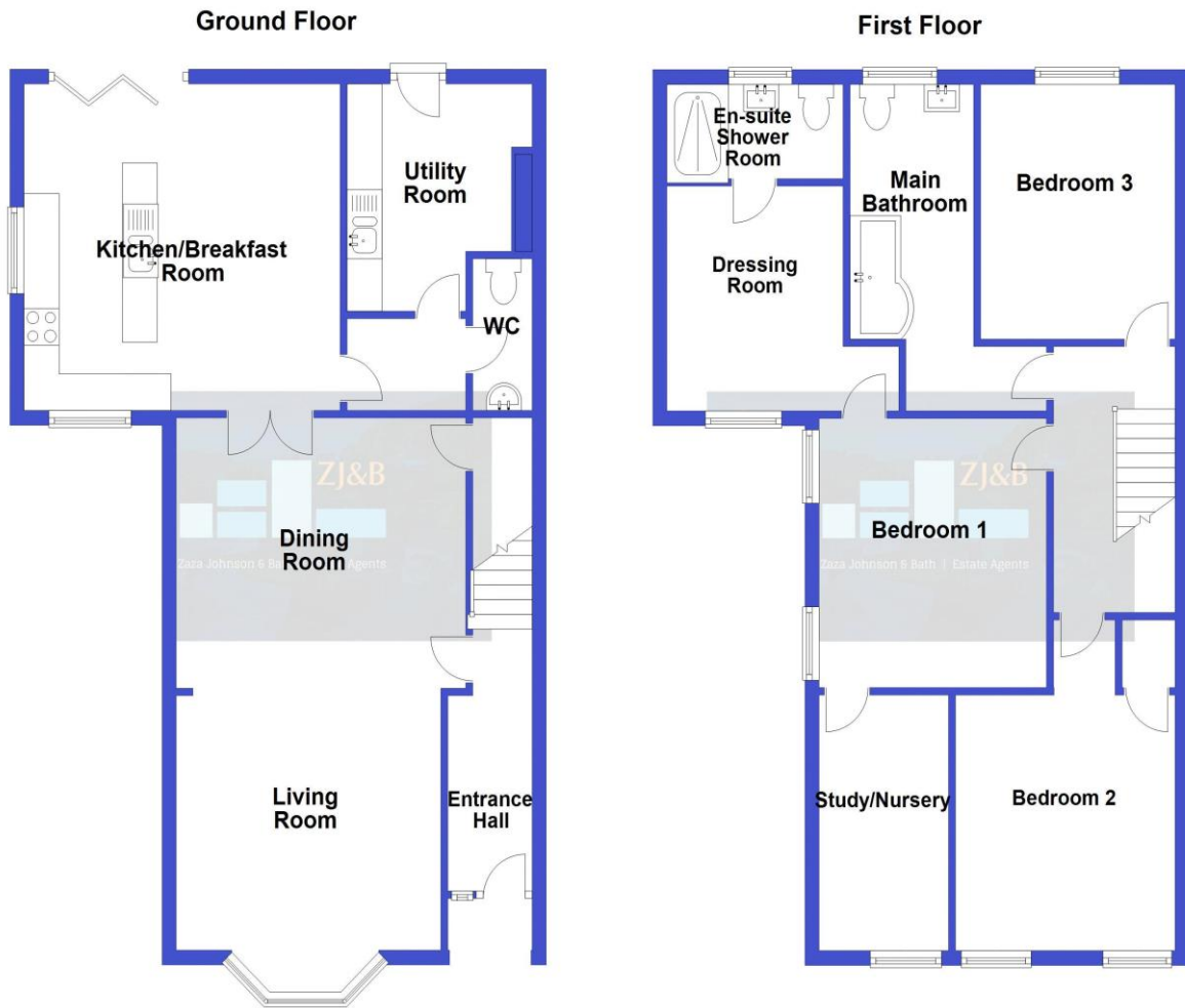
FLOOR PLANS FOR GUIDANCE ONLY
