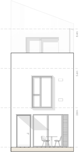
FRONT 1:50
