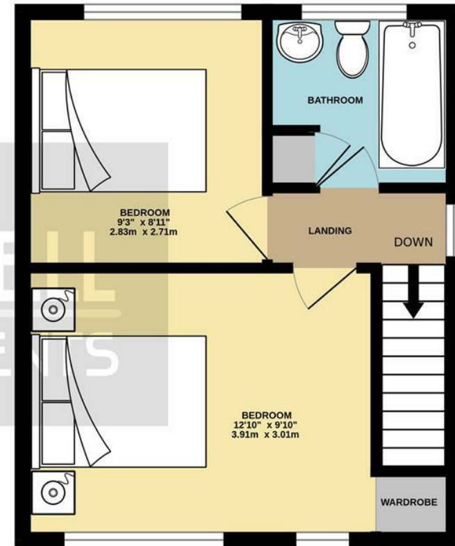
TOTAL FLOOR AREA : 621 sq.ft. (57.7 sq.m.) approx.
