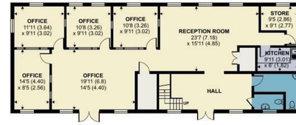
GROUND FLOOR 2
