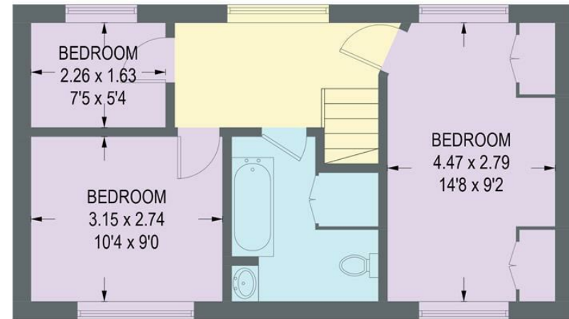
FIRST FLOOR 40.7 SQ M / 438 SQ FT
