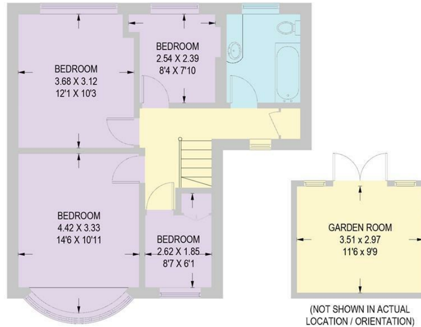
FIRST FLOOR 48.8 SQ M / 525 SQ FT
