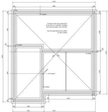
PROPOSED FOUNDATION PLAN
