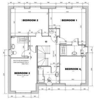
PROPOSED FIRST FLOOR PLAN
