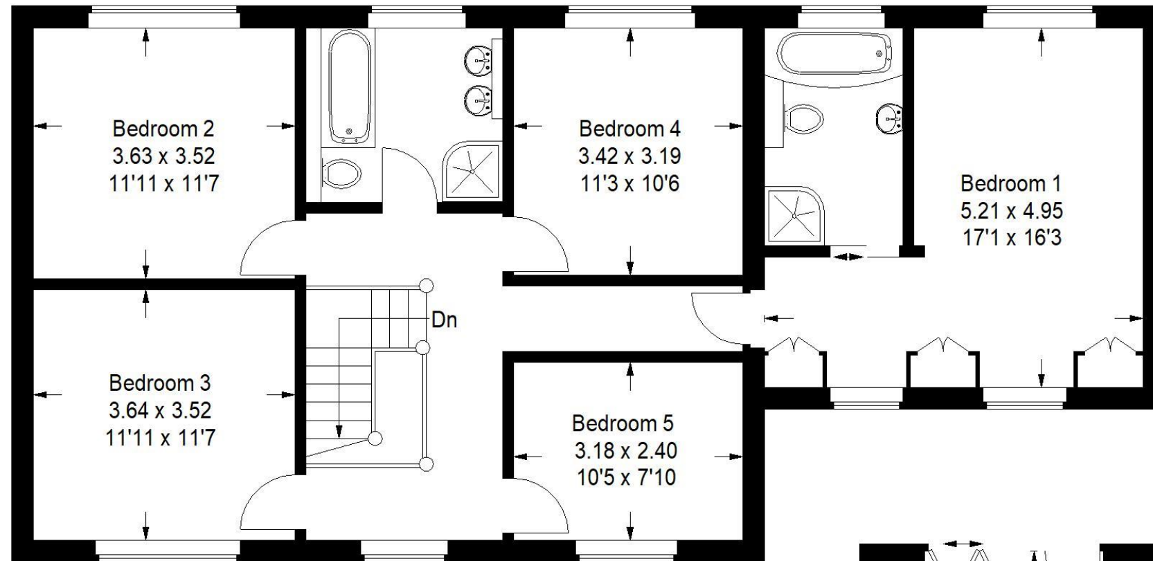
First Floor
