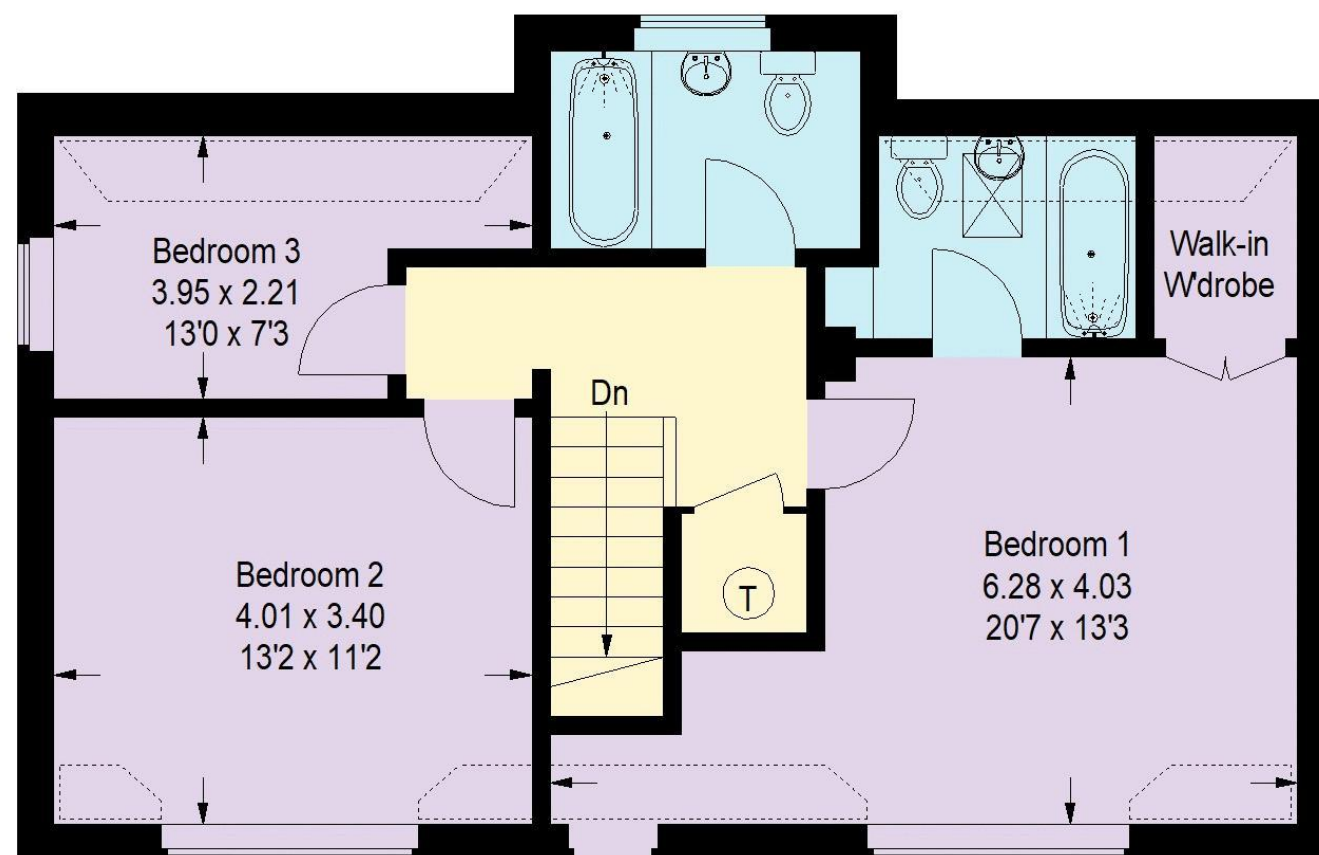
First Floor
