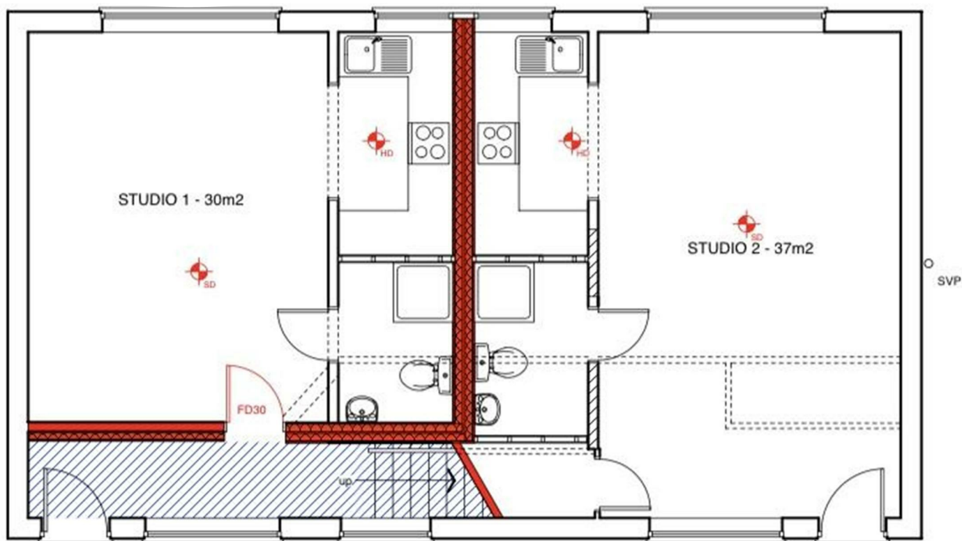
PROPOSED FIRST FLOOR PLAN 1:50 @ A2
