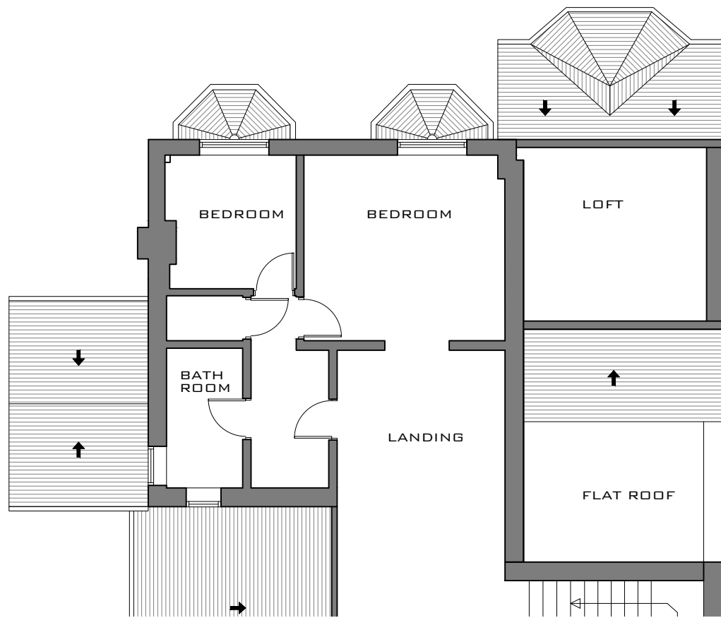
FIRST FLOOR PLAN EXISTING
