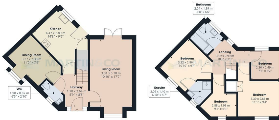
Floor 0 Building 1
