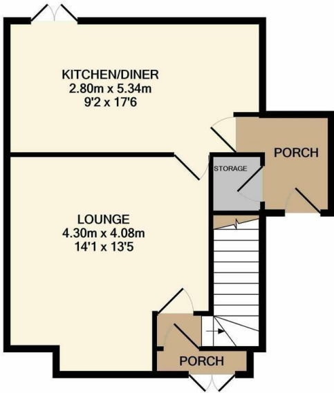
GROUND FLOOR APPROX. FLOOR AREA 41.9 SQ.M. (451 SQ.FT.)
