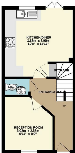
GROUND FLOOR 30.6 sq.m. (329 sq.ft.) approx.
