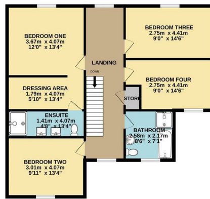
1ST FLOOR 89.2 sq.m. (960 sq.ft.) approx.
