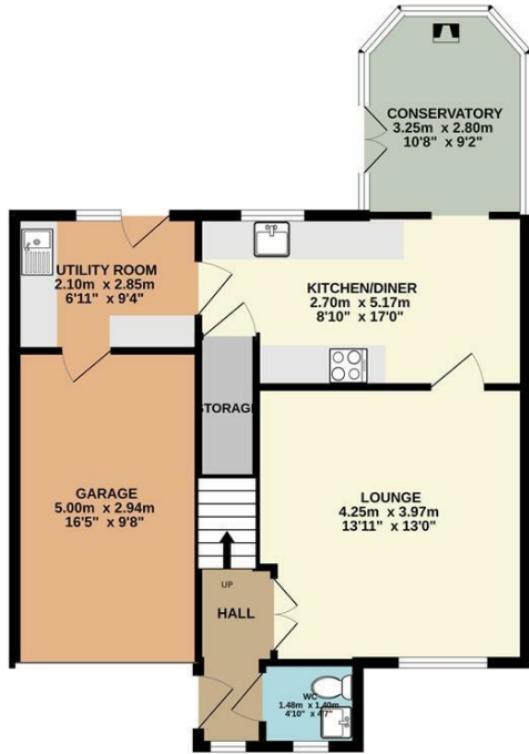
GROUND FLOOR 67.6 sq.m. (728 sq.ft.) approx.
