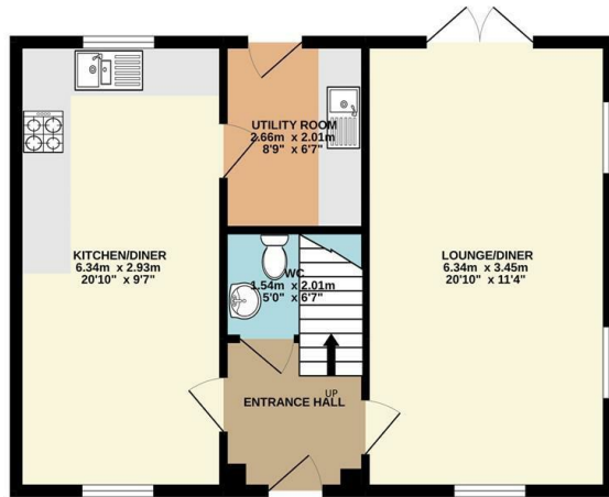
GROUND FLOOR 52.9 sq.m. (570 sq.ft.) approx.
