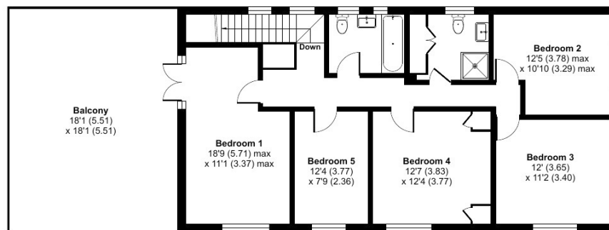
FIRST FLOOR
