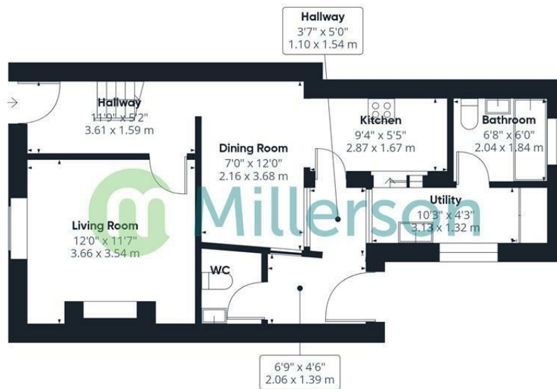
Floor 0 Building 1
