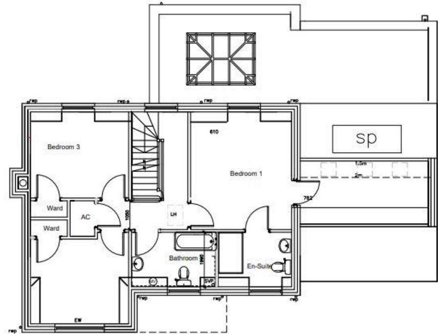
PLOT 1 FIRST FLOOR PLAN 1-50 (76sqm-818 sqft)
