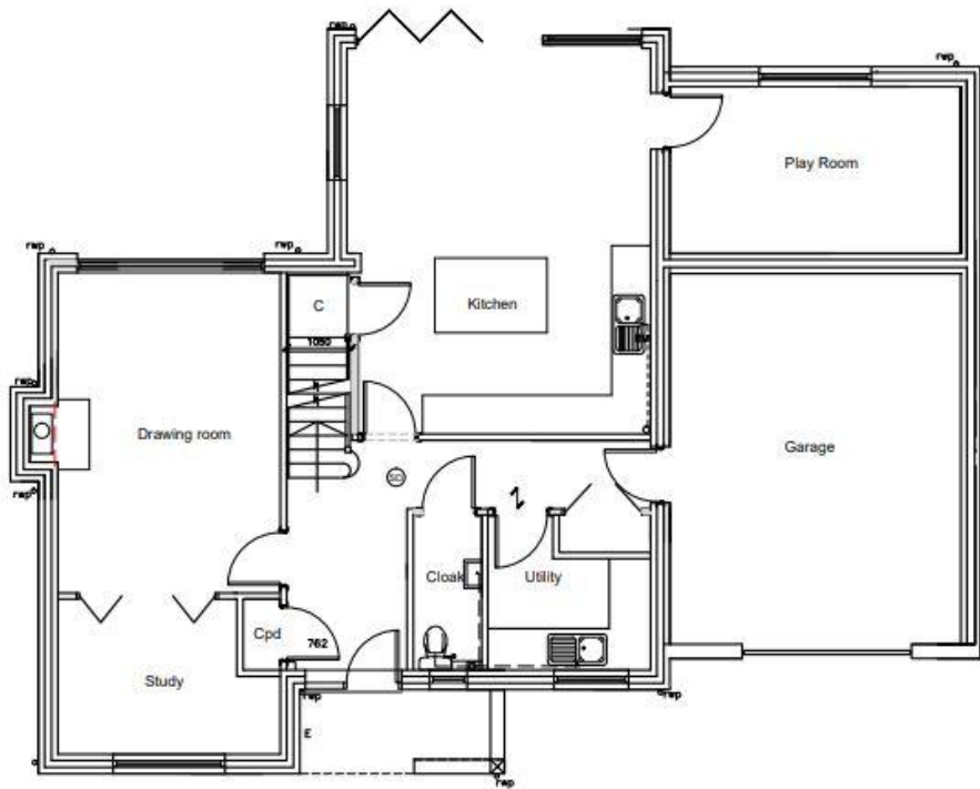
PLOT 1 GROUND FLOOR PLAN 1-50 (127sqm-1364 sqft)
