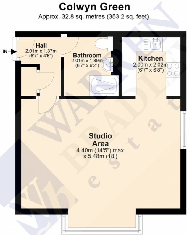
Total area: approx. 32.8 sq. metres (353.2 sq. feet)
