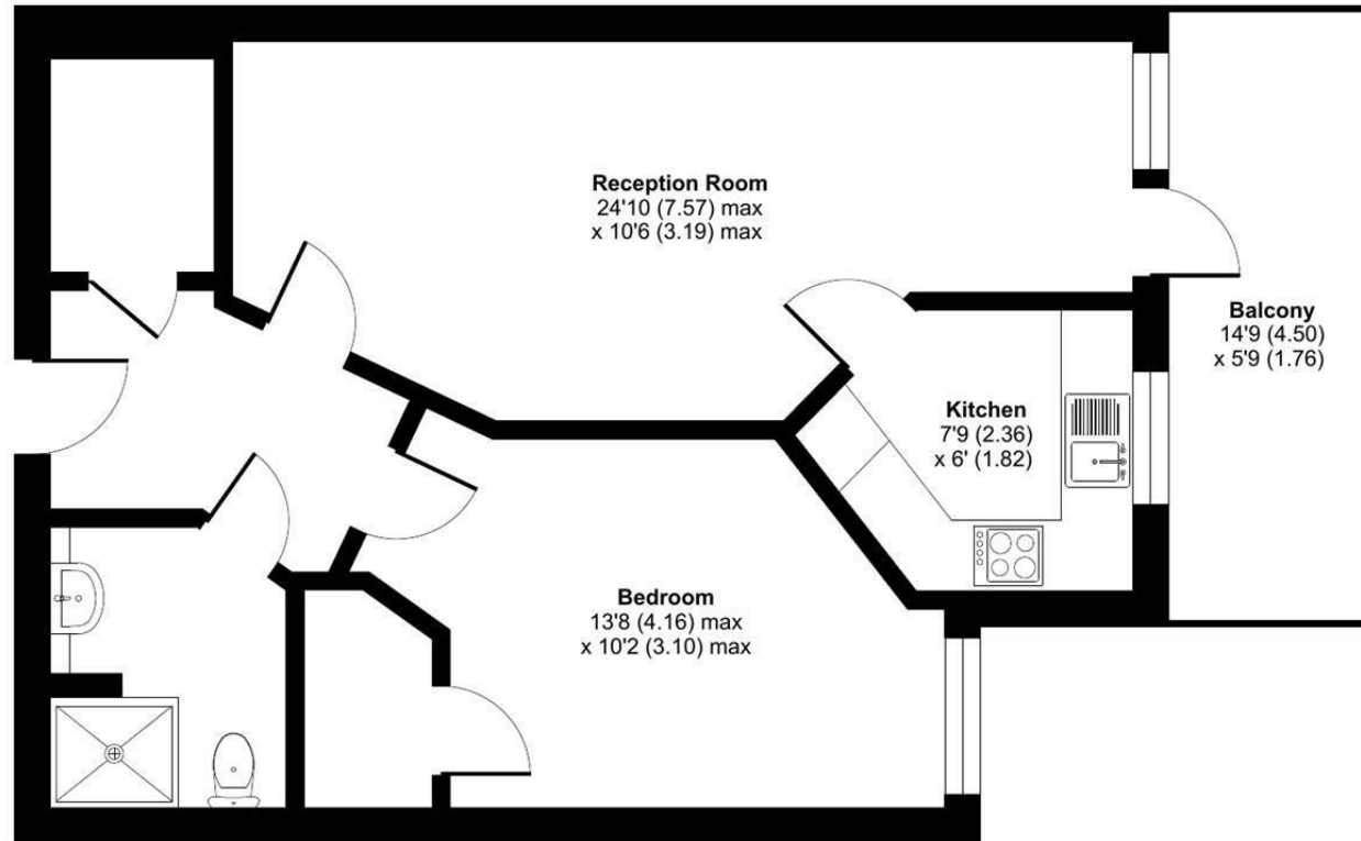
FIRST FLOOR
