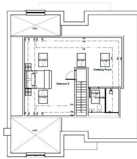
Proposed Loft Floor Plan Unit 1
