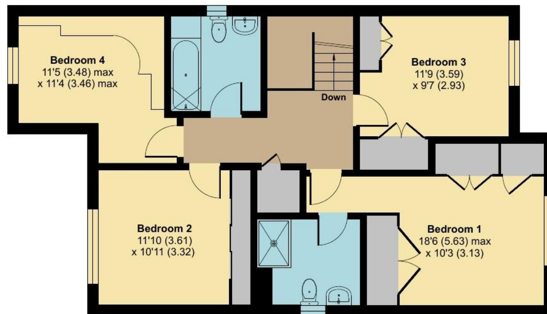
FIRST FLOOR
