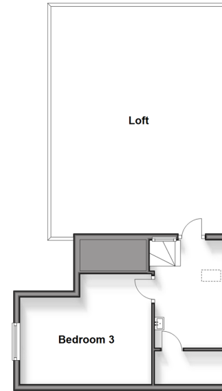
Second Floor Approx. 23.5 sq. metres (253.4 sq. feet)
