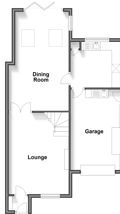
Ground Floor Approx. 62.6 sq. metres (673.4 sq. feet)
