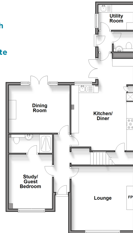
Ground Floor Approx. 85.2 sq. metres (917.6 sq. feet)
