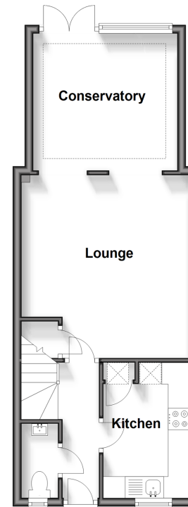
Ground Floor Approx. 442.8 sq. feet
