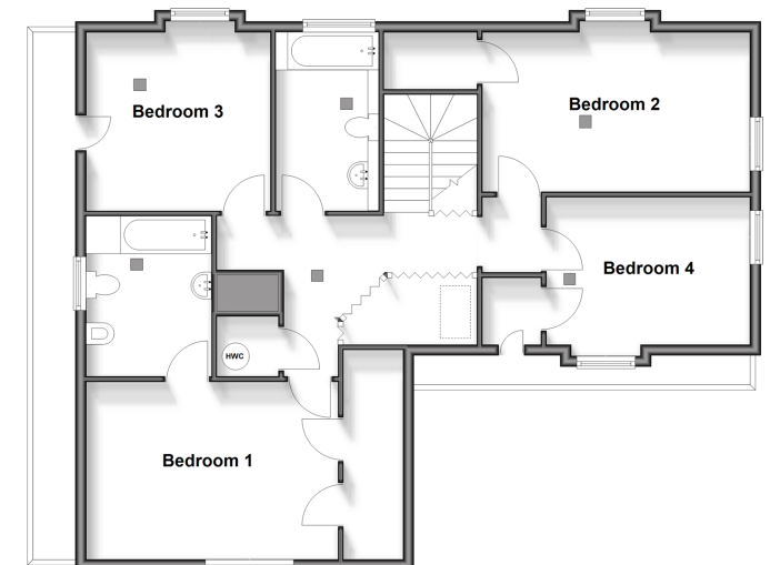
First Floor Approx. 95.5 sq. metres (1028.5 sq. feet)
