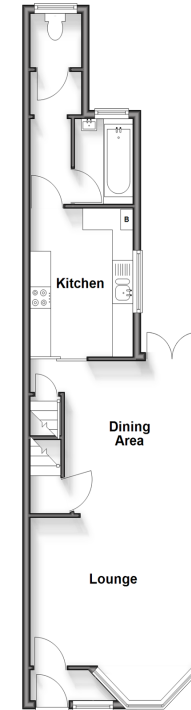
Split Level Ground Floor Approx. 47.9 sq. metres (515.4 sq. feet)
