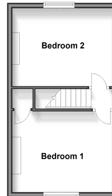
First Floor Approx. 28.6 sq. metres (307.6 sq. feet)
